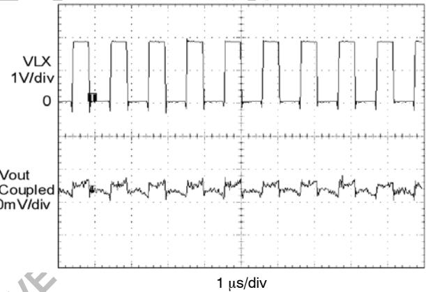
Figure 19. Heavy-Load PWM Switching Waveform ( V_{in} = 3.6\text{ V} , V_{out} = 1.5\text{ V} , I_{out} = 300\text{ mA} )
